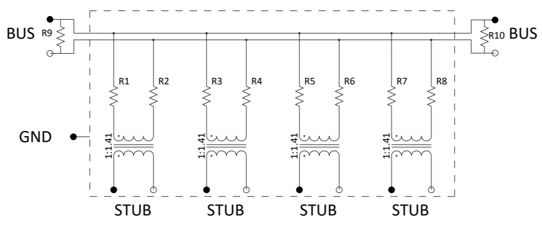
SCHMATIC DIAGRAM
